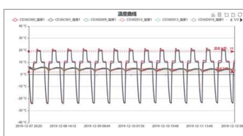
ISTA 7D HOT/COID +2°C TO +8°C FOR 72:00HRS
