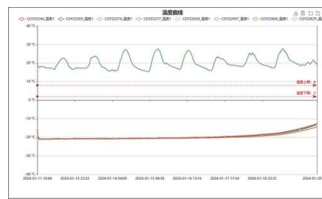
ISTA 7D HOT -25°C TO -15°C FOR 72:00HRS
